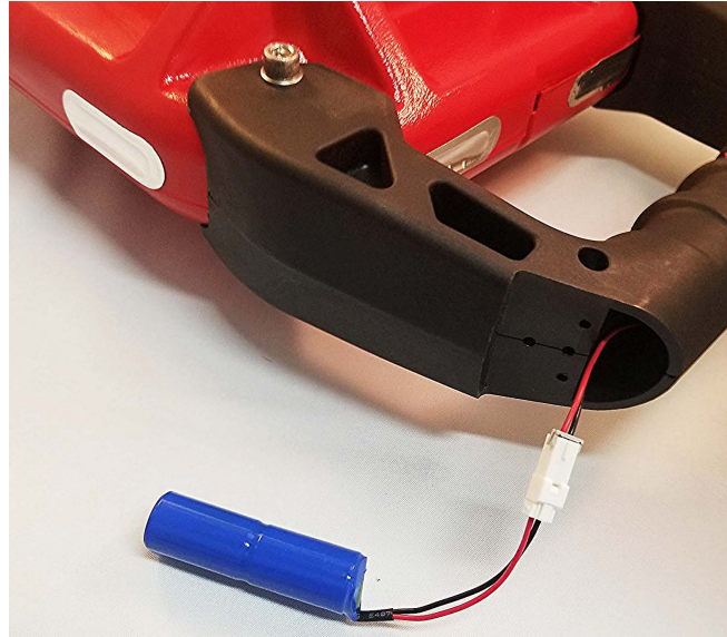
2.) Connect the battery to the connector in the handle
