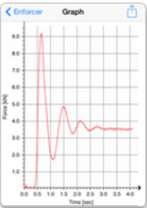
Graph of 4 second event, with option to export to CSV file.
